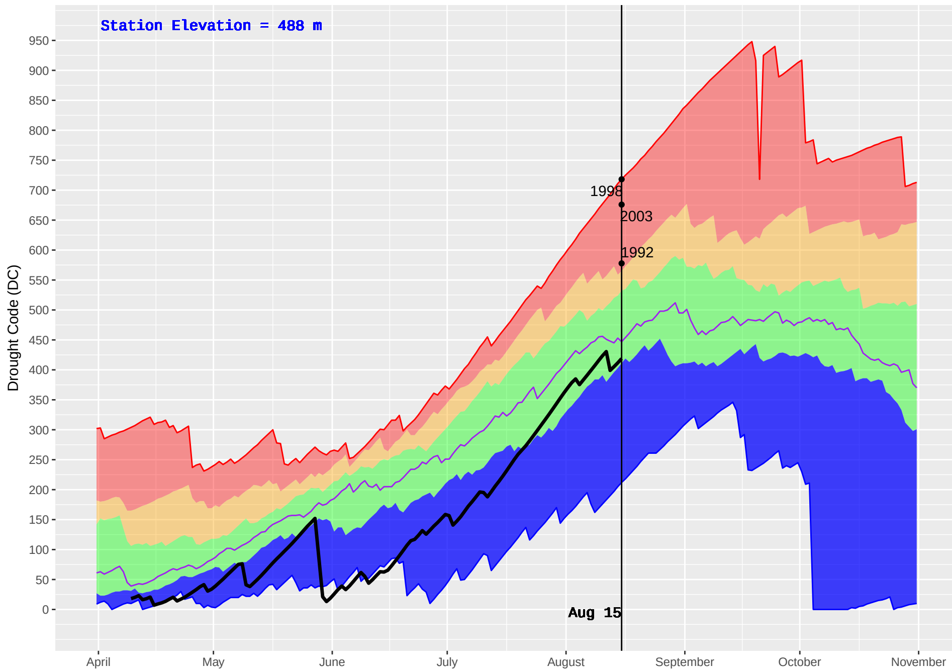
MABEL LAKE 2 (362) : Historical (1987–2016) and Current (2018) Daily Drought Code (DC)
