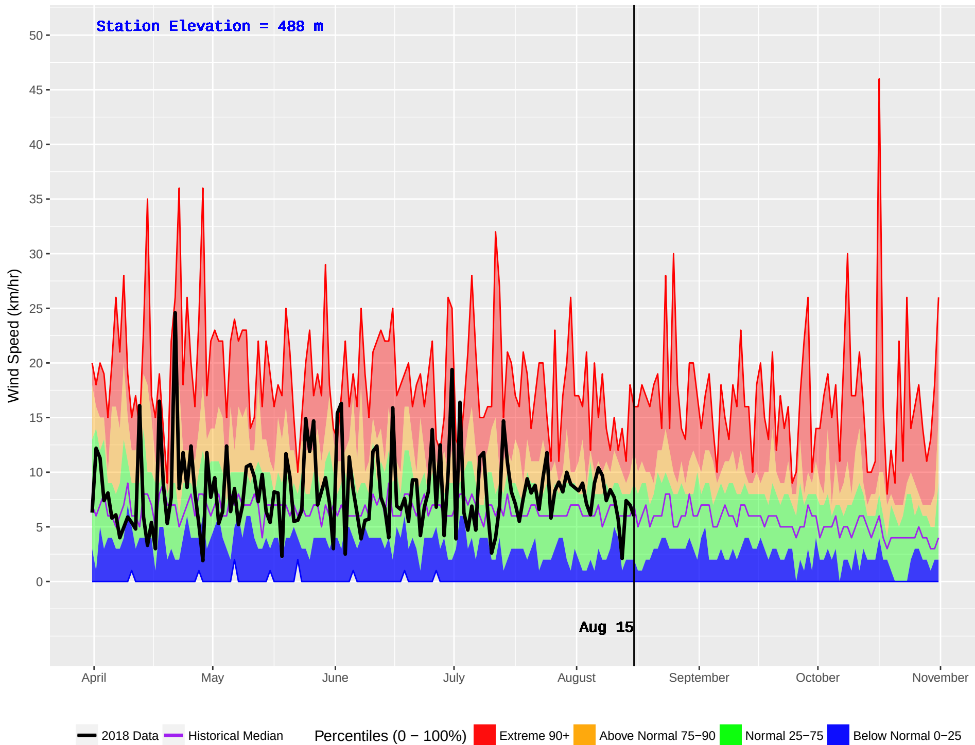
MABEL LAKE 2 (362) : Historical (1987–2016) and Current (2018) Daily Wind Speed
