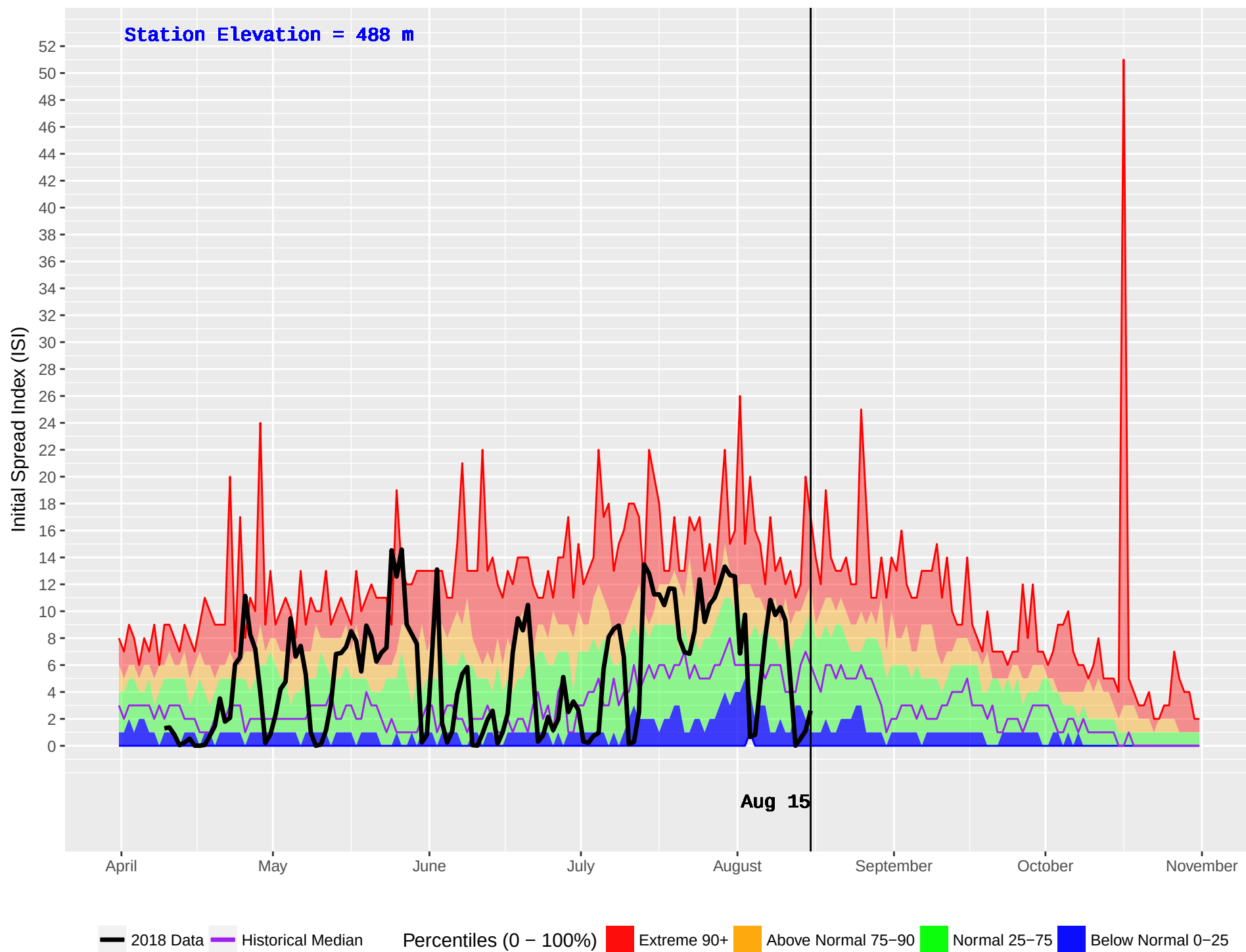
MABEL LAKE 2 (362) : Historical (1987–2016) and Current (2018) Daily Initial Spread Index (ISI)
