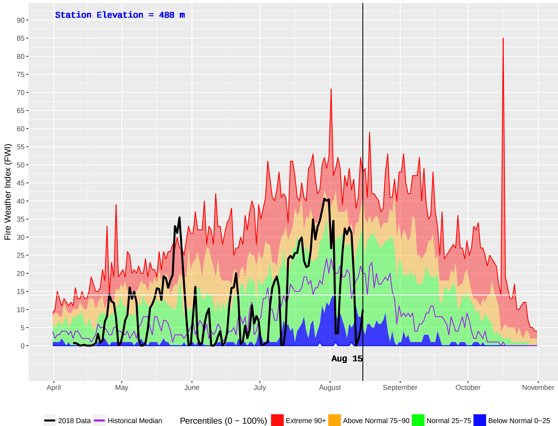
MABEL LAKE 2 (362) : Historical (1987–2016) and Current (2018) Daily Fire Weather Index (FWI)
