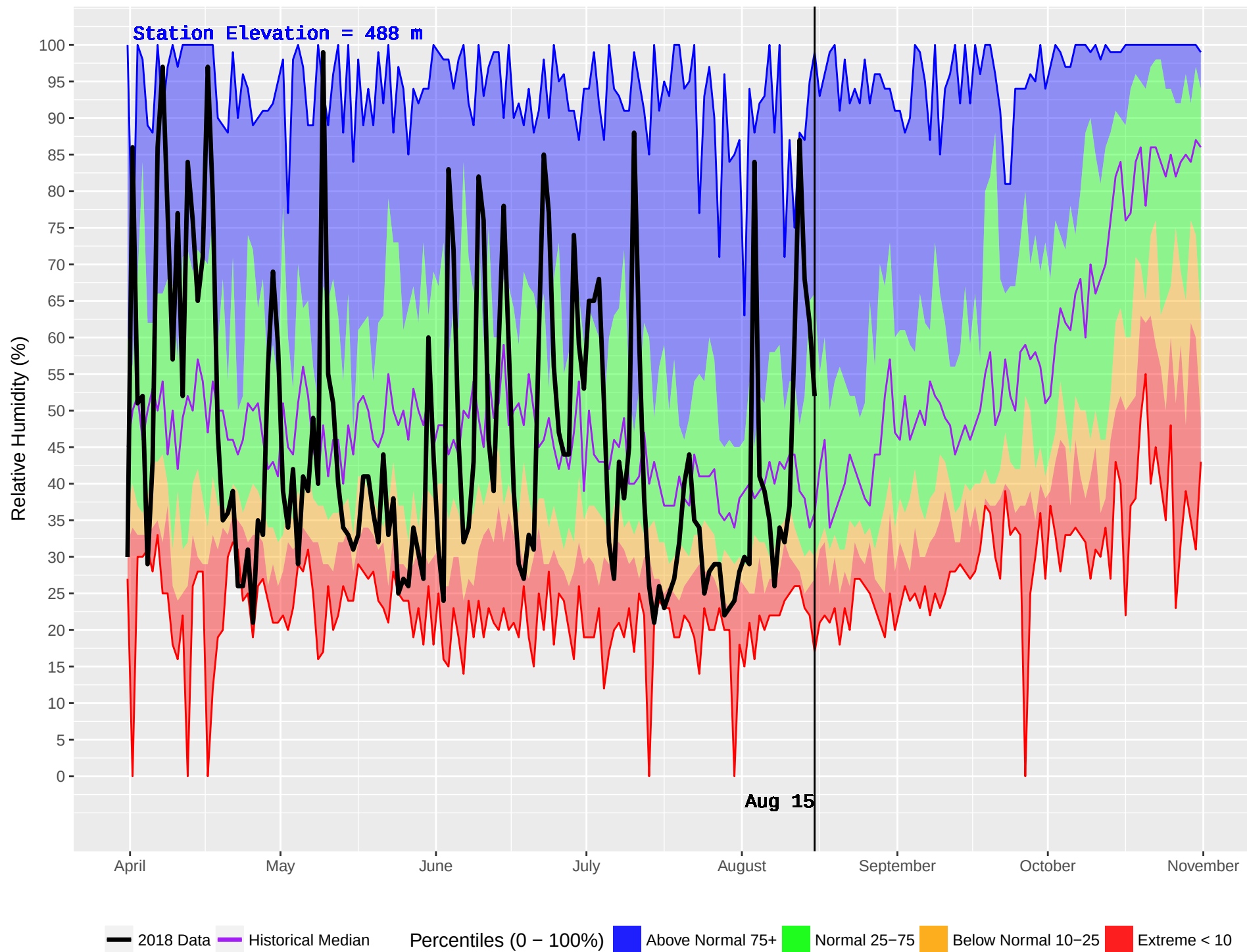
MABEL LAKE 2 (362) : Historical (1987–2016) and Current (2018) Daily Relative Humidity
