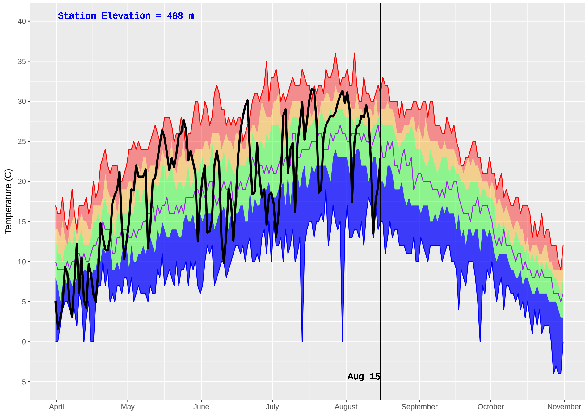
MABEL LAKE 2 (362) : Historical (1987–2016) and Current (2018) Daily Temperature
