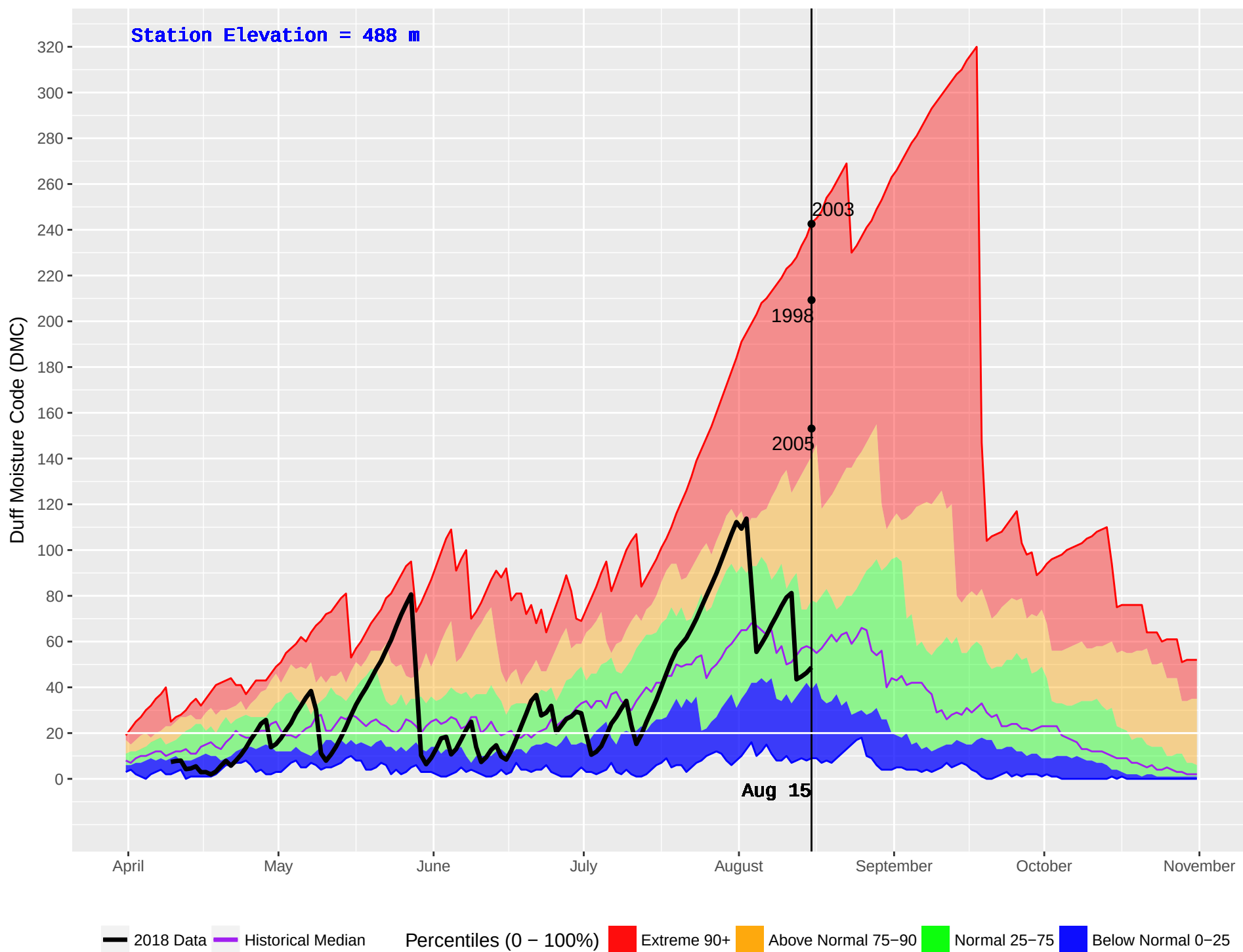
MABEL LAKE 2 (362) : Historical (1987–2016) and Current (2018) Daily Duff Moisture Code (DMC)
